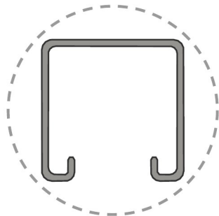
UNICANAL 41.3 × 41.3 mm
